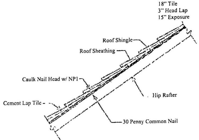
Section of Lap Tile
