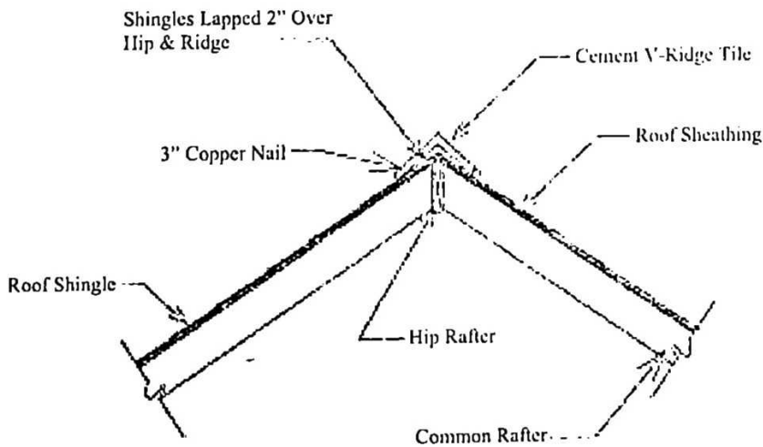
Section of Ridge/Hip
