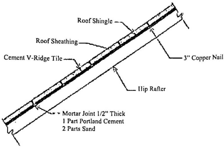
Section of Butted Tile
